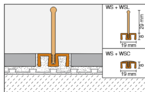
Schlüter®-SHOWERPROFILE-WS
